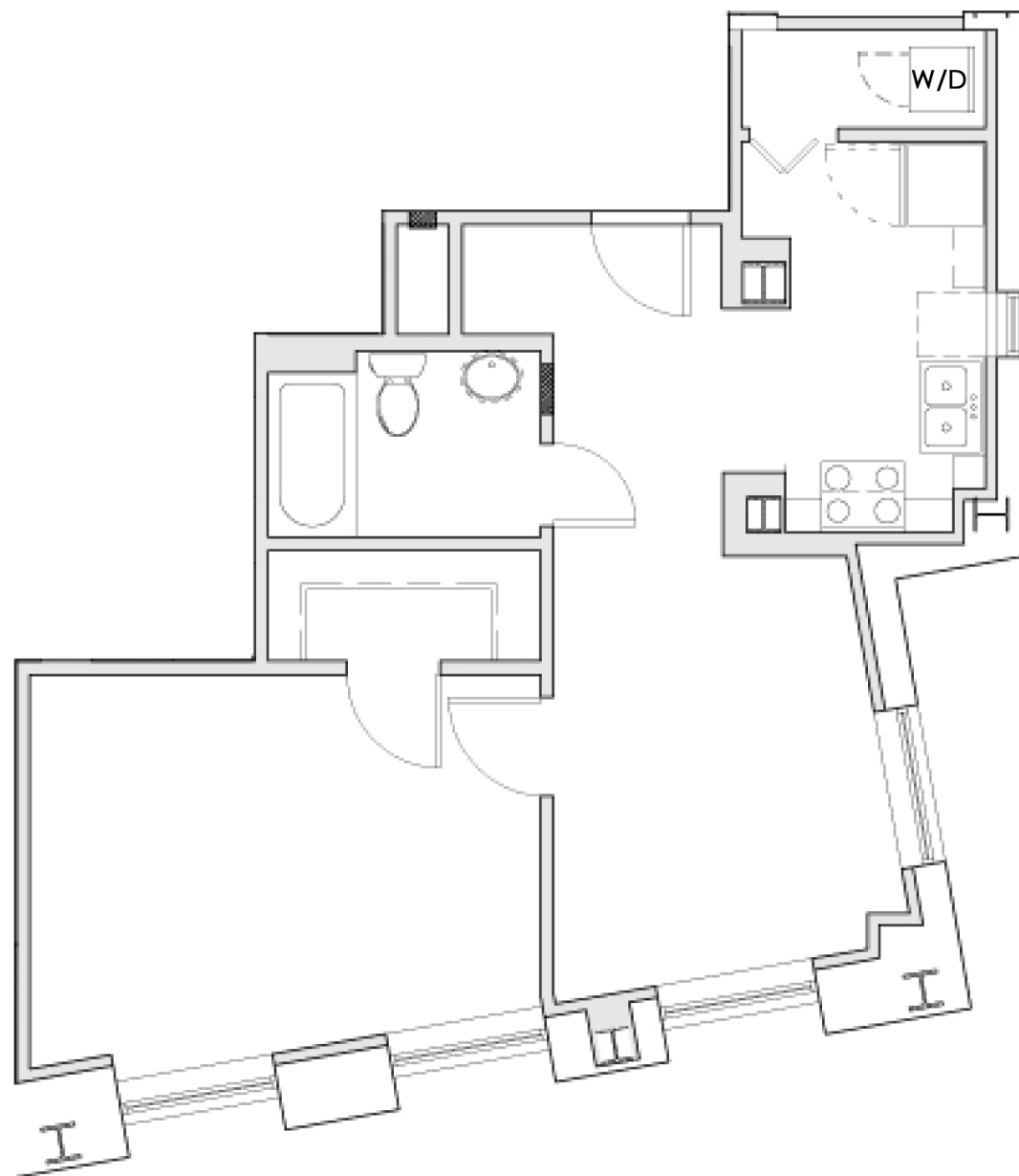
UNIT 01 AT FLOORS 20 & 21
